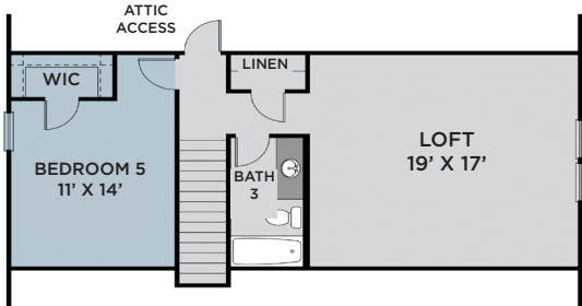
OPTIONAL SECOND FLOOR W/ BED 5
